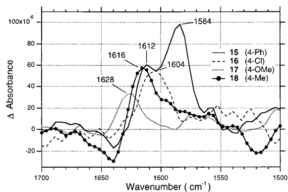
Figure 2. TRIR difference spectra observed over the first 1.0 \mu\text{s} following laser photolysis (266 nm, 10 ns, 0.4 mJ) of pyridinium salts 15–18 in argon-saturated acetonitrile- d_3 .
